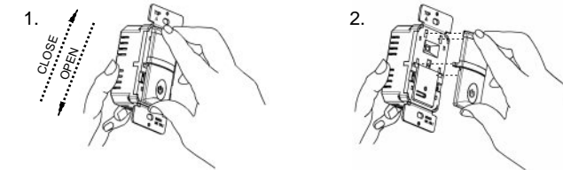
Slide down top cover to release Line up tabs and slide up to attach
